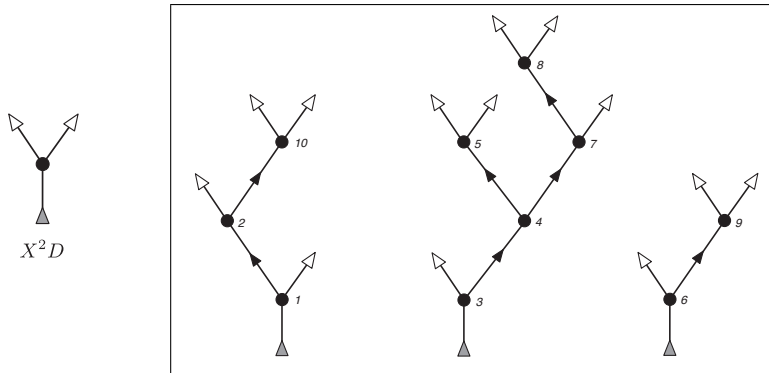
FIGURE 13. The basic gate \mathbb{Y} associated with X^2D (left) and a corresponding diagram (right box).
