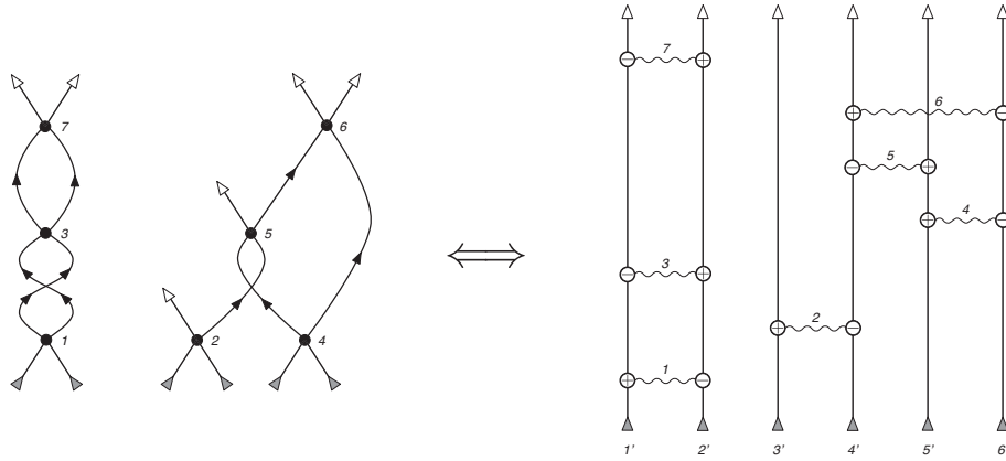
FIGURE 9. The scaffolding representation of an X^2 D^2 graph (and the induced canonical labelling of lines).
